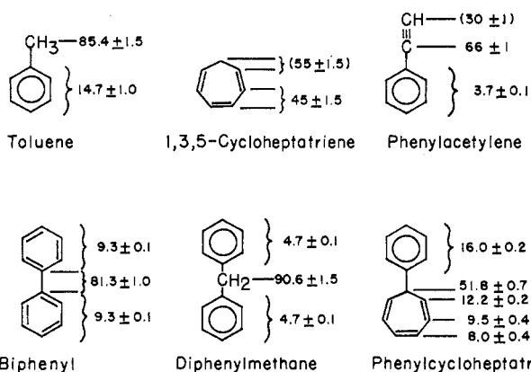
Figure 2. Distribution of ^{14}\text{C} in major products formed by the irradiation of solid benzene with 5 keV ^{14}\text{C}^+ ions.
